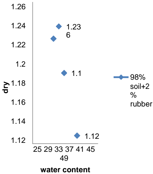
Figure 1: water content Vs dry density
